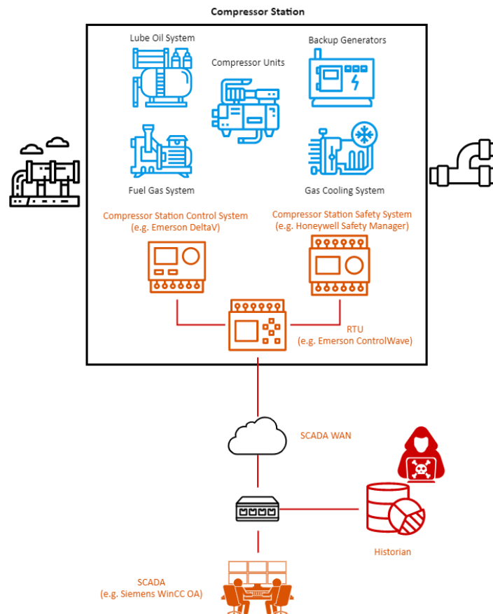
Figure 12 – Natural Gas Transport System
